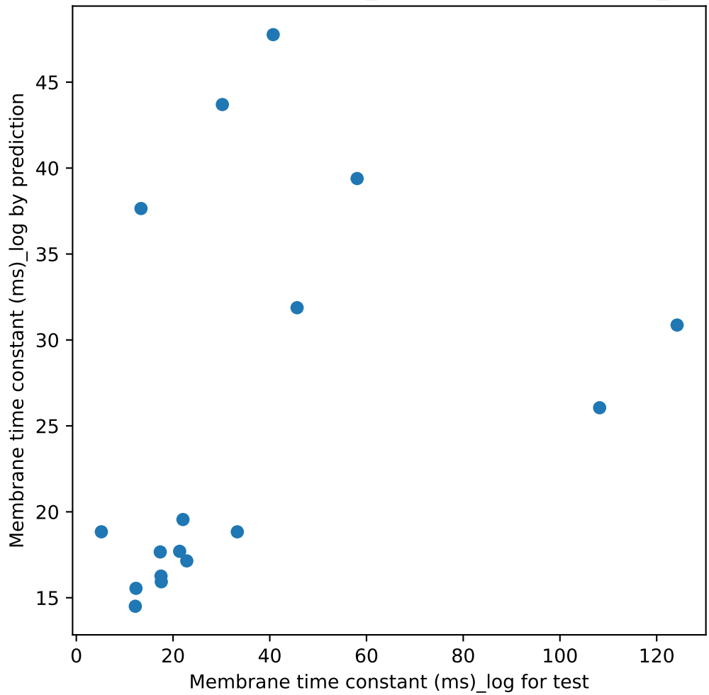
prediction of Membrane time constant (ms)_log by embs alpha 0.2 l1_ratio 0.8 MAE 17.733
